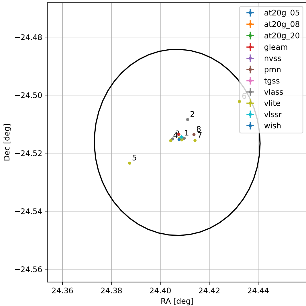
4FGL J0137.6-2430
