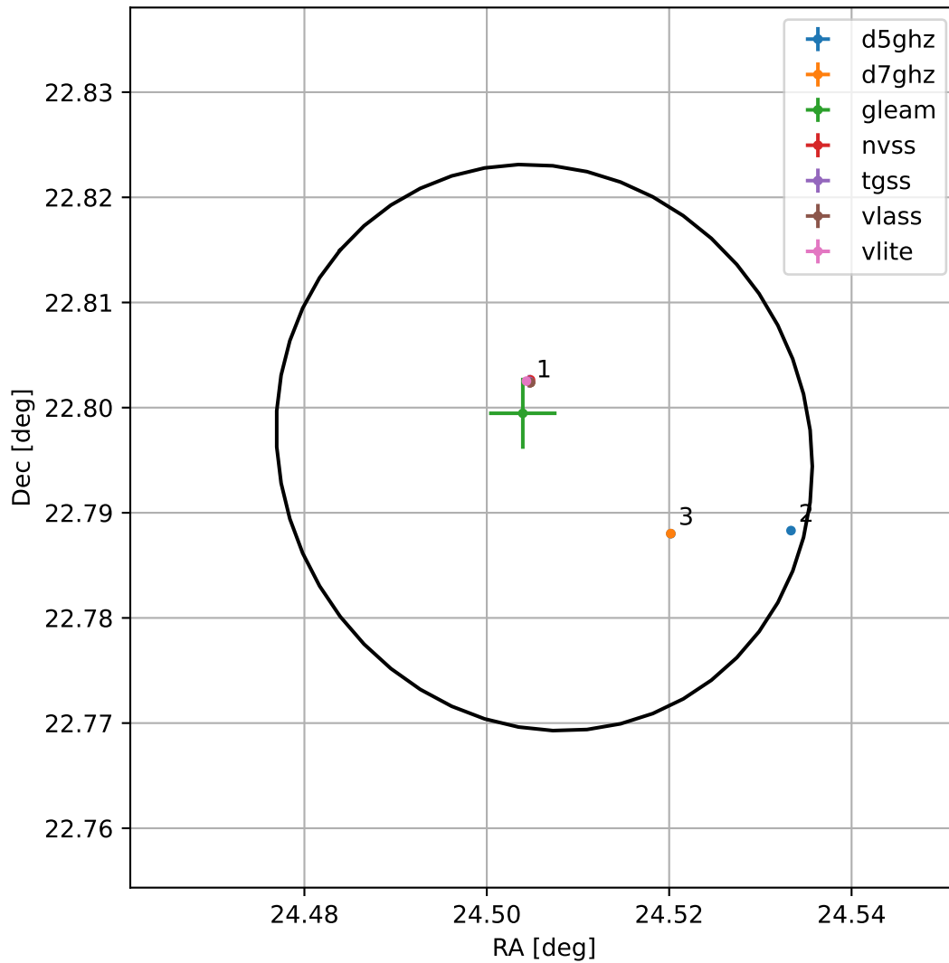
4FGL J0138.0+2247
