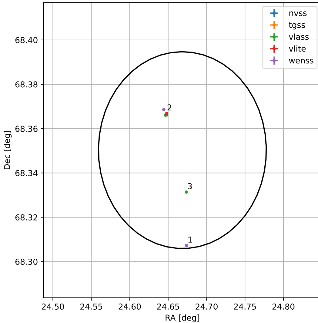
4FGL J0138.6+6821
