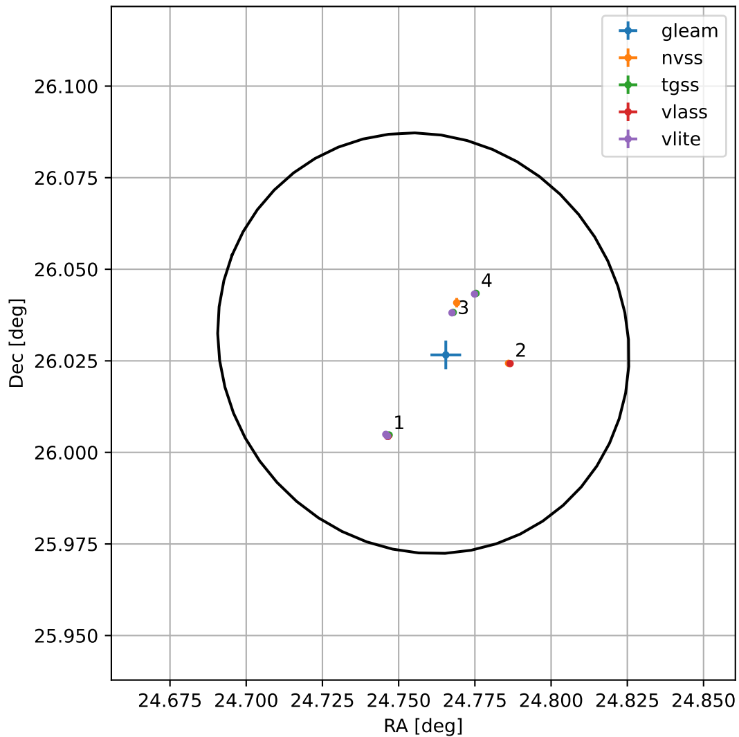
4FGL J0139.0+2601
