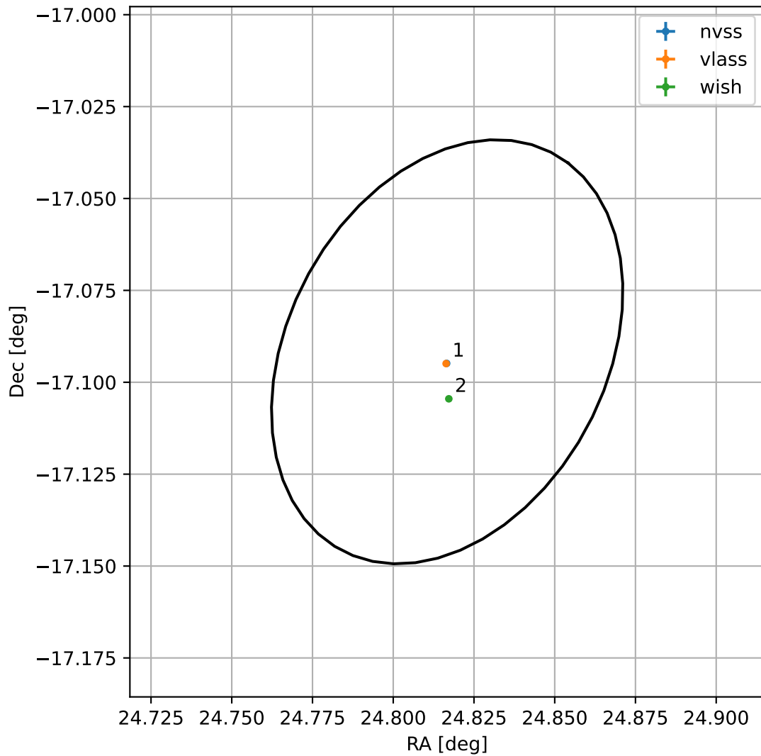
4FGL J0139.2-1705
