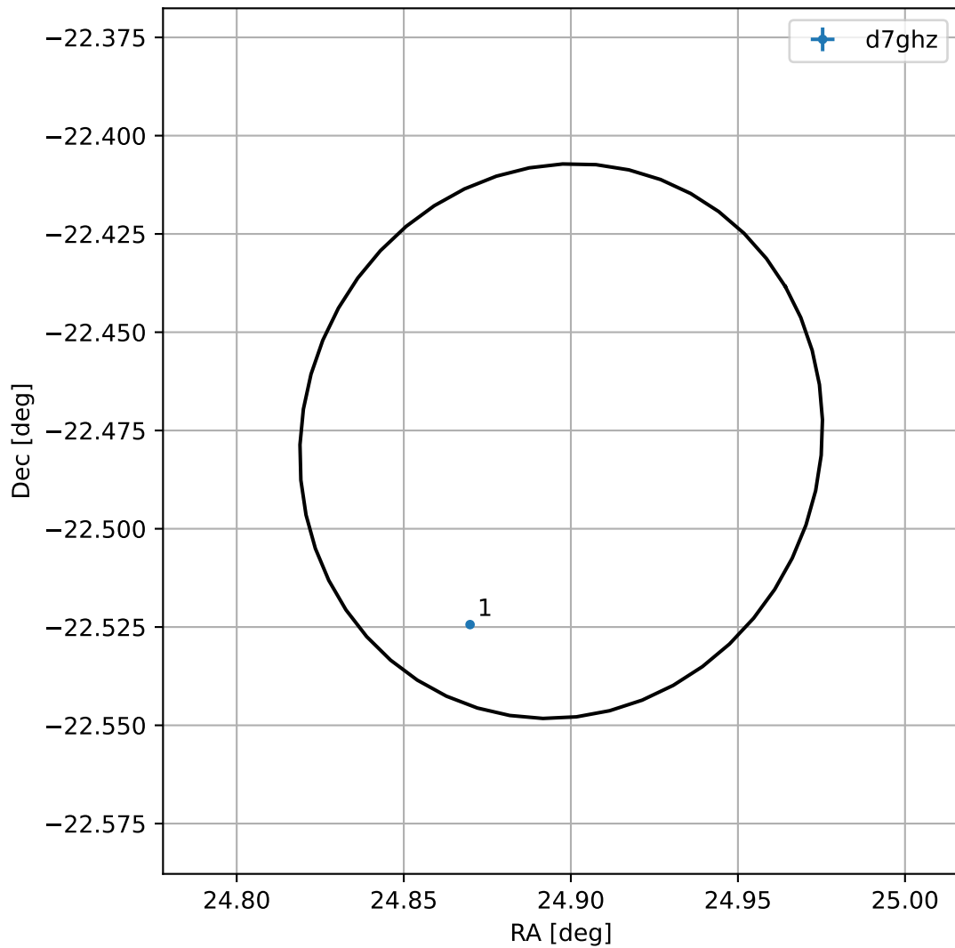
4FGL J0139.5-2228
