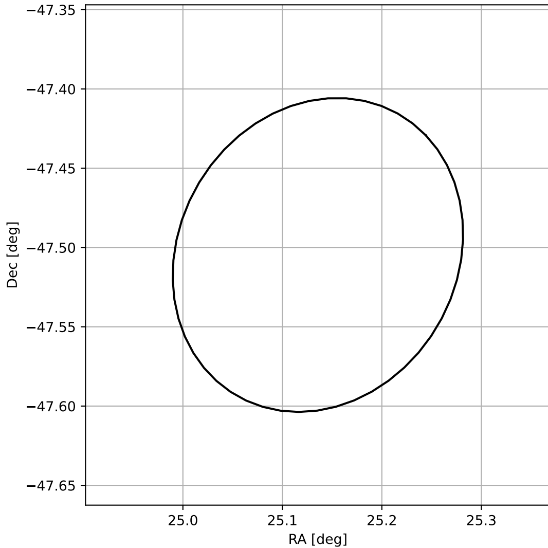
4FGL J0140.5-4730
