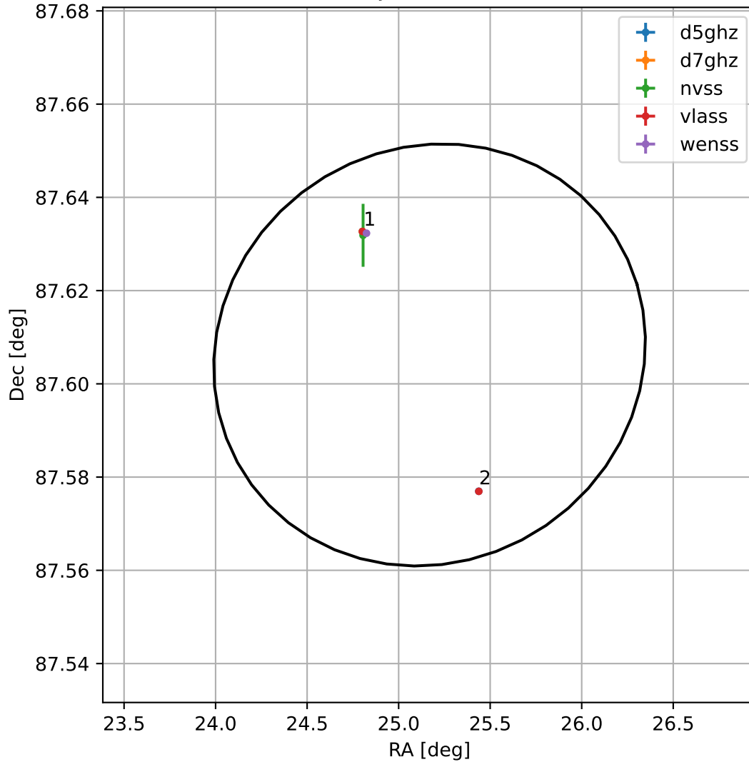
4FGL J0140.6+8736
