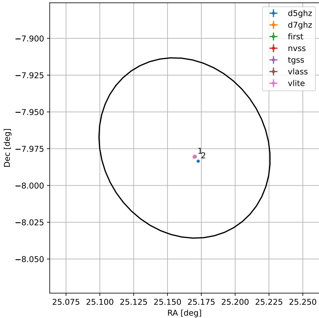
4FGL J0140.6-0758
