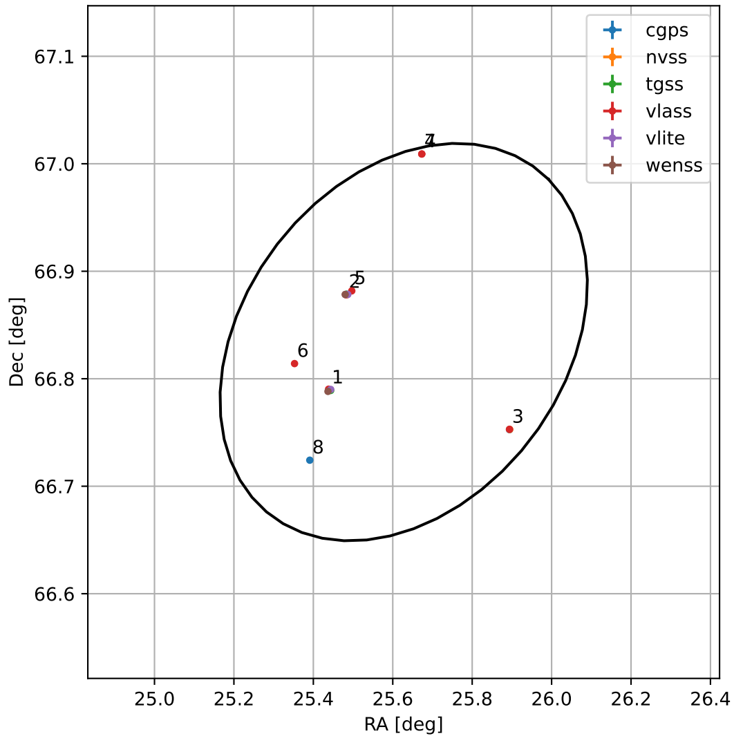
4FGL J0142.5+6650
