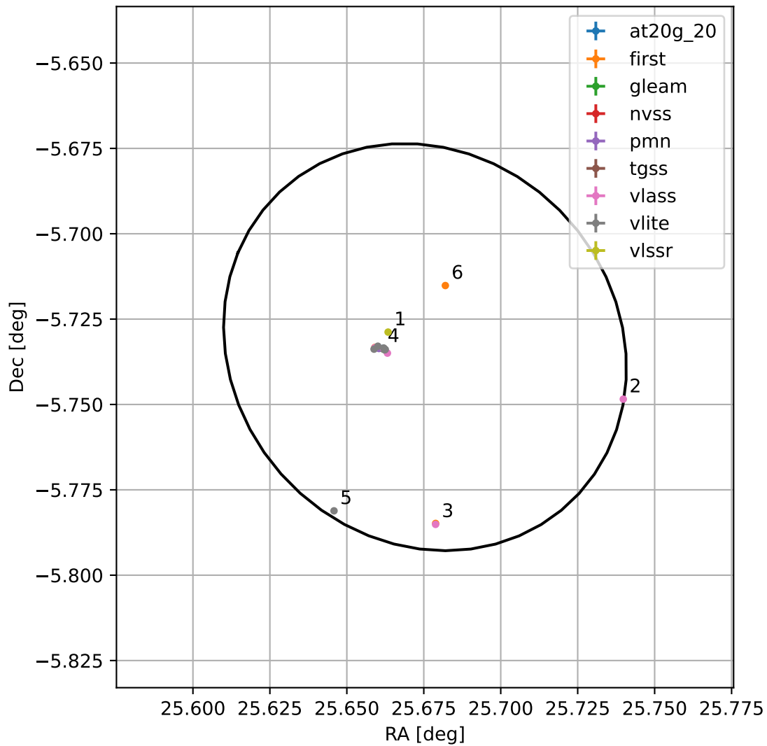
4FGL J0142.7-0543
