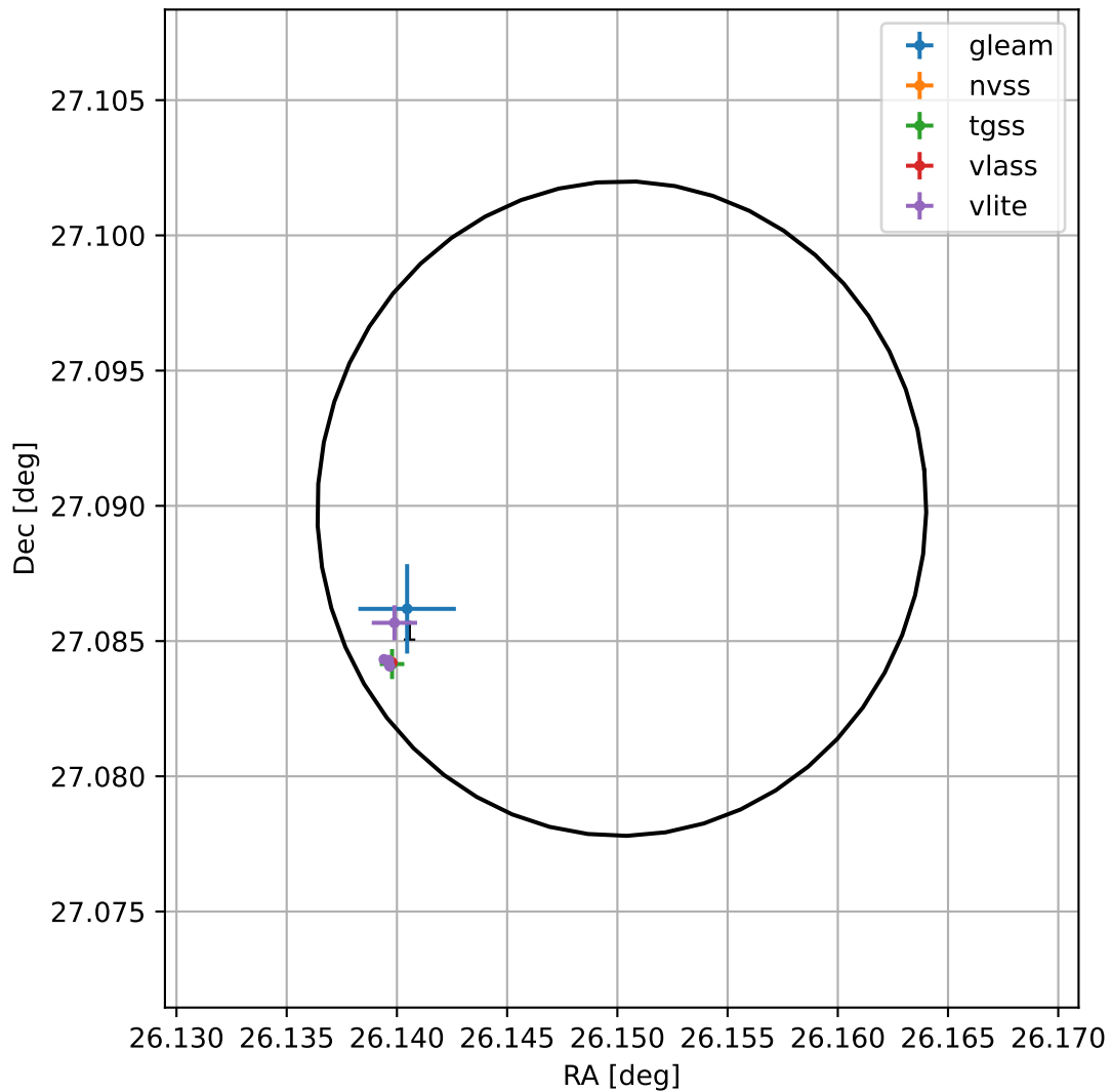
4FGL J0144.6+2705
