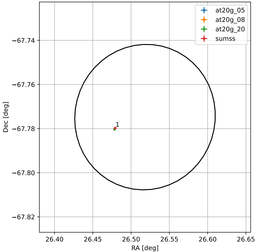
4FGL J0146.0-6746
