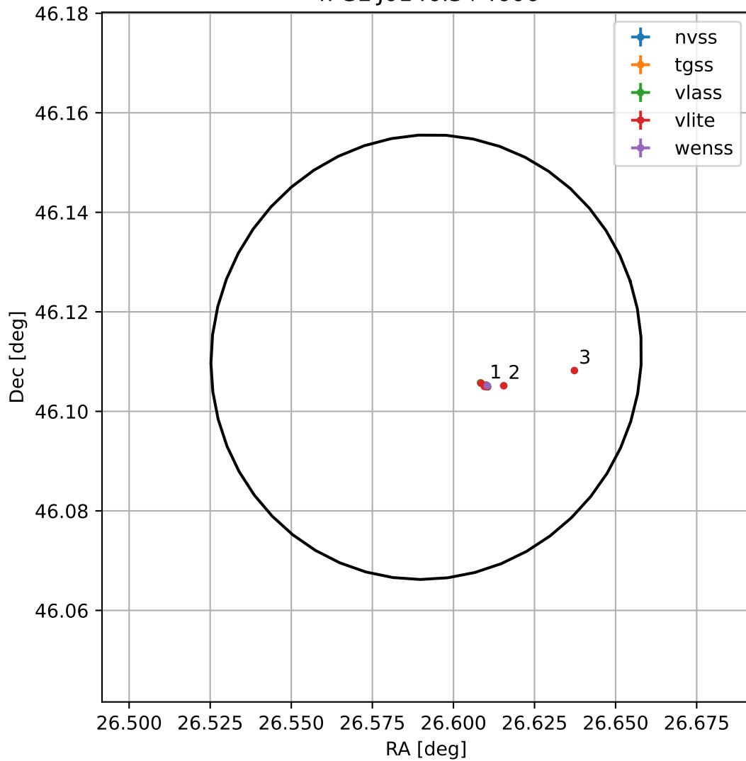
4FGL J0146.3+4606
