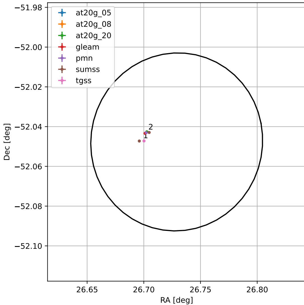
4FGL J0146.9-5202
