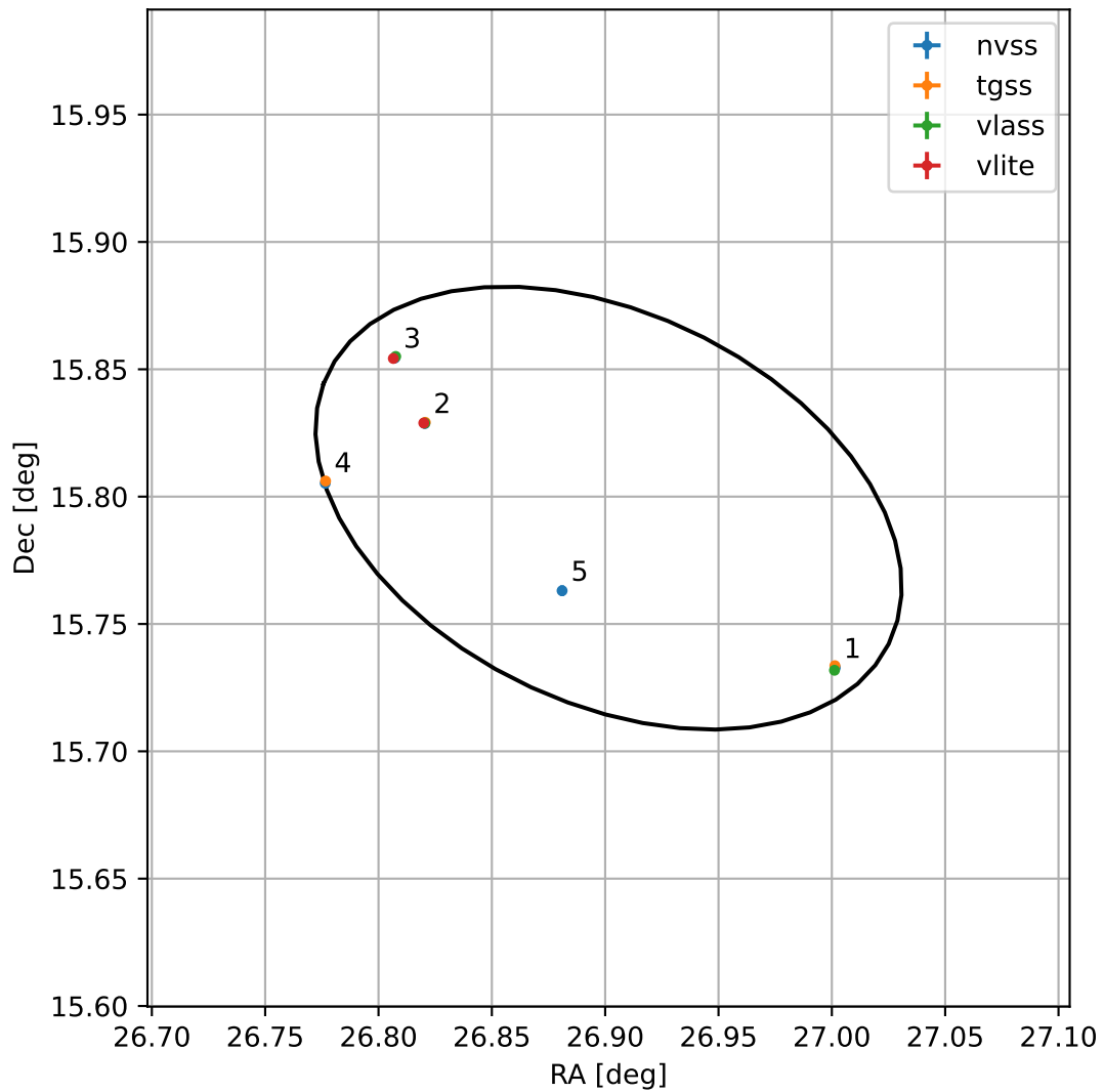
4FGL J0147.6+1547
