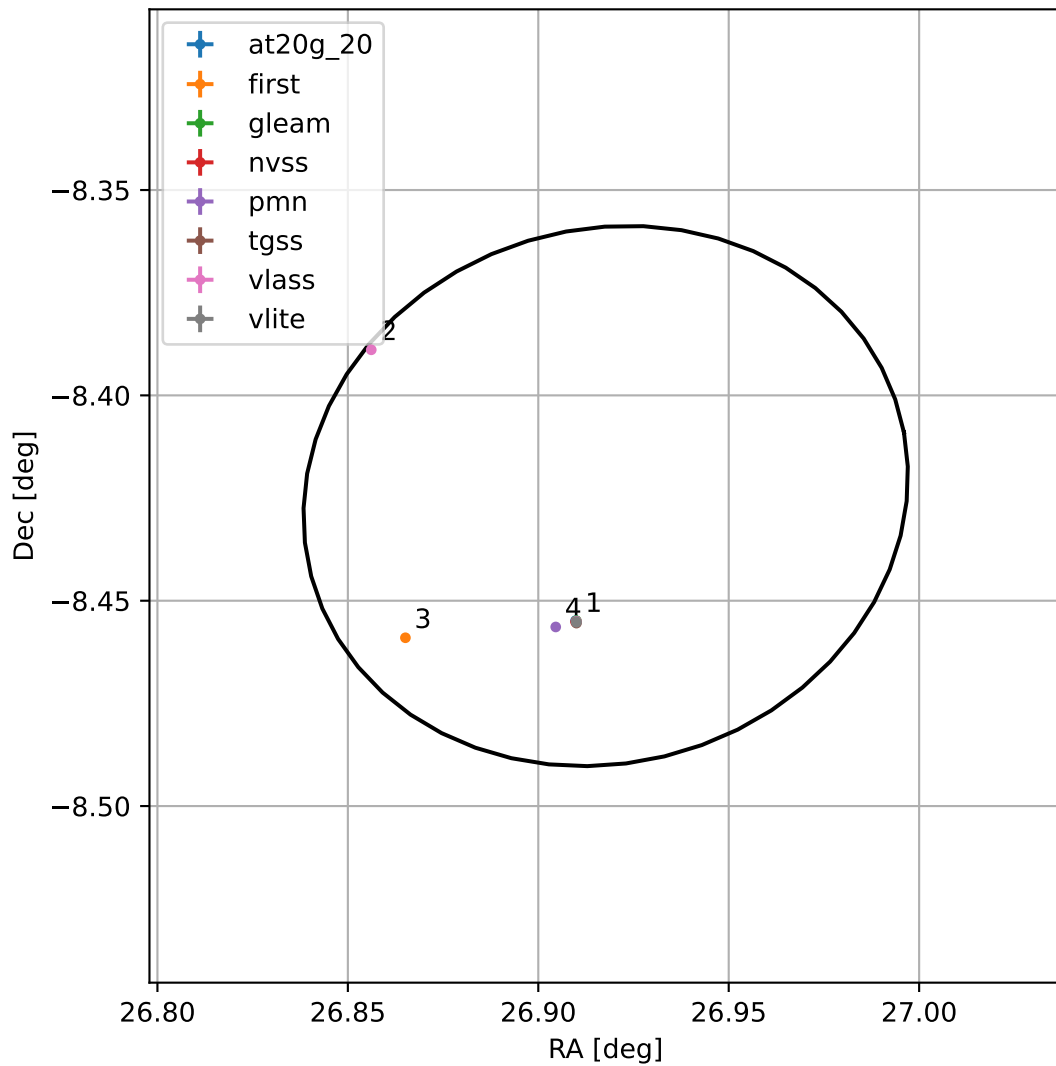
4FGL J0147.6-0825
