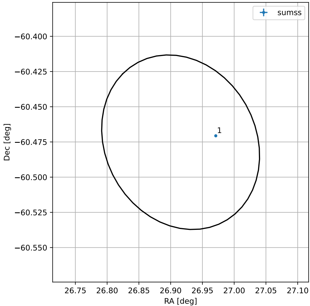
4FGL J0147.6-6028
