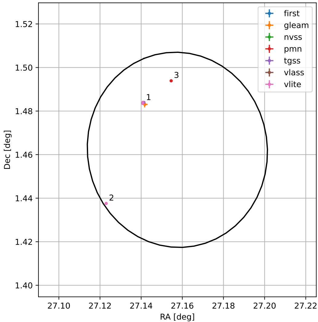
4FGL J0148.6+0127
