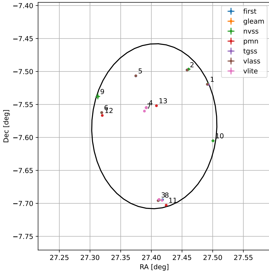
4FGL J0149.6-0734
