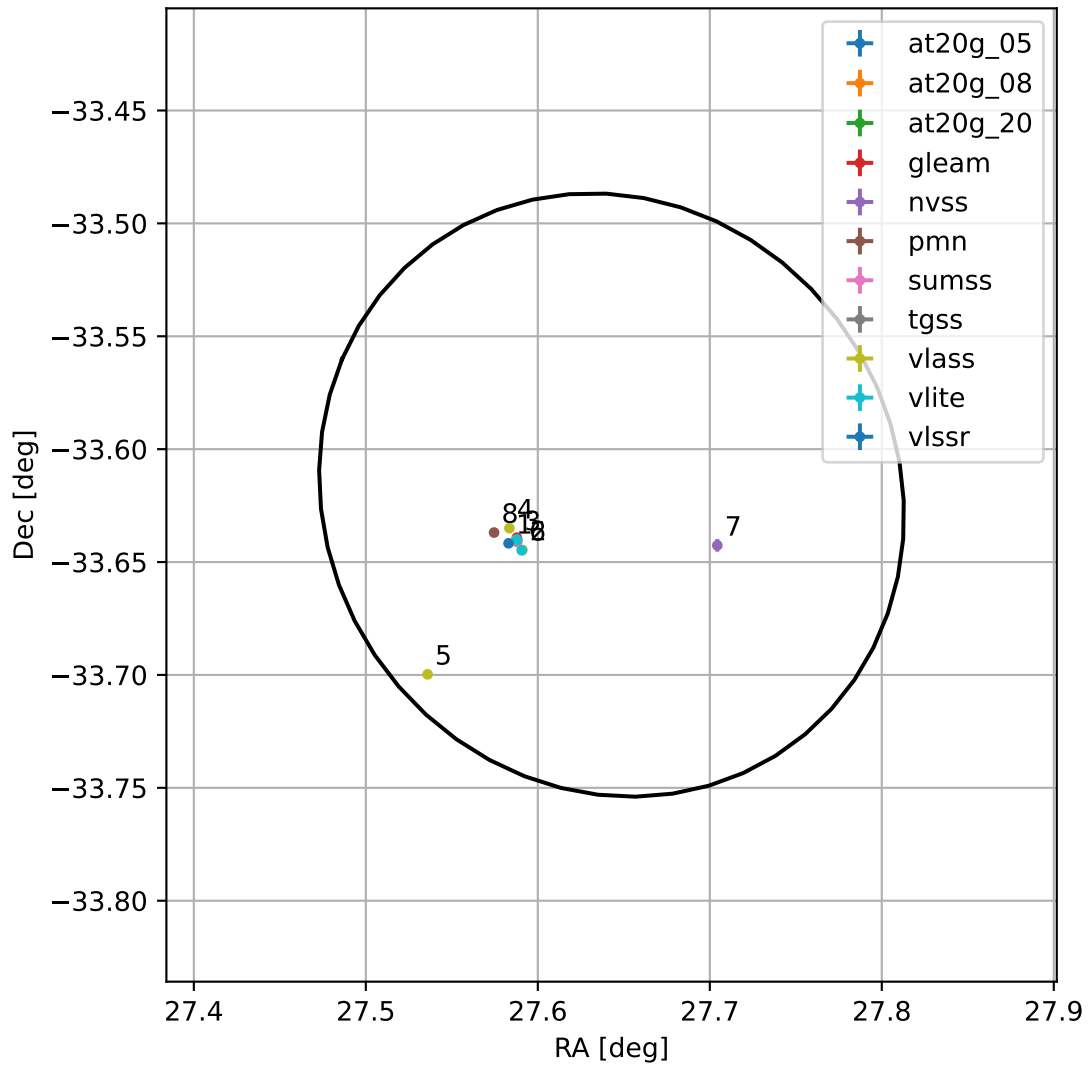
4FGL J0150.5-3337
