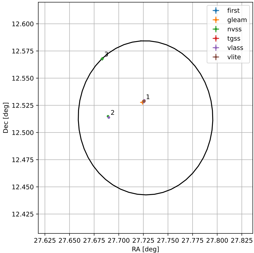
4FGL J0150.9+1230
