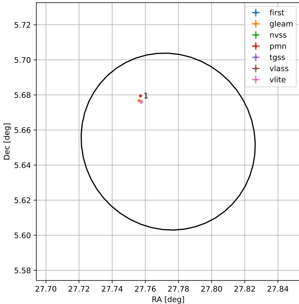
4FGL J0151.0+0539
