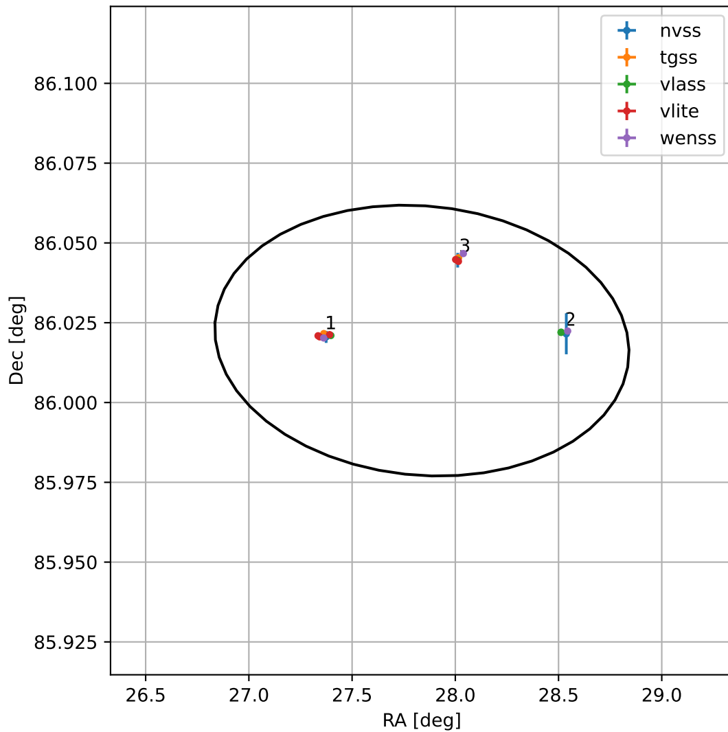
4FGL J0151.3+8601
