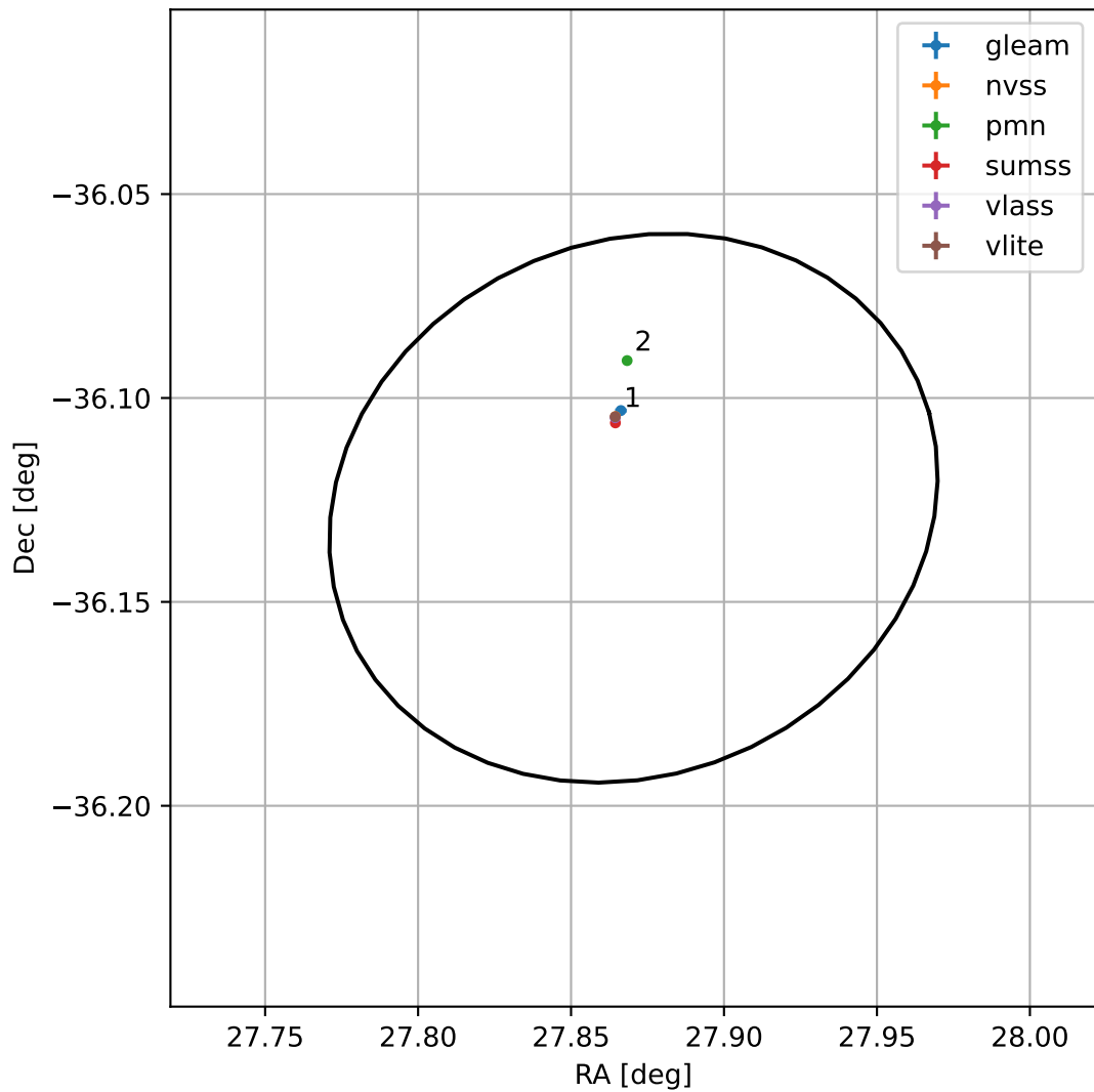
4FGL J0151.4-3607
