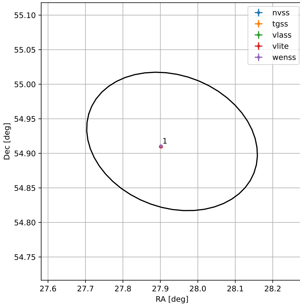
4FGL J0151.7+5455
