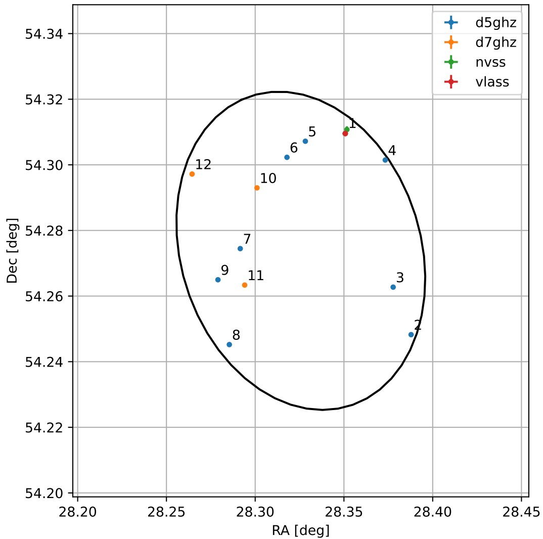
4FGL J0153.3+5416
