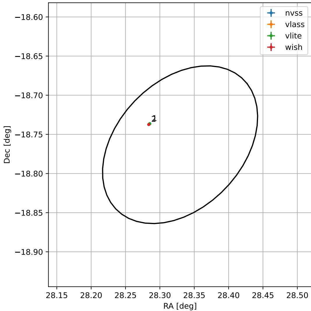
4FGL J0153.3-1845
