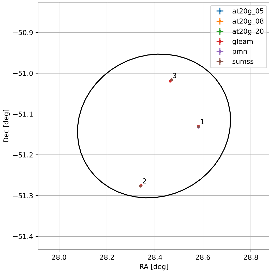
4FGL J0153.5-5107
