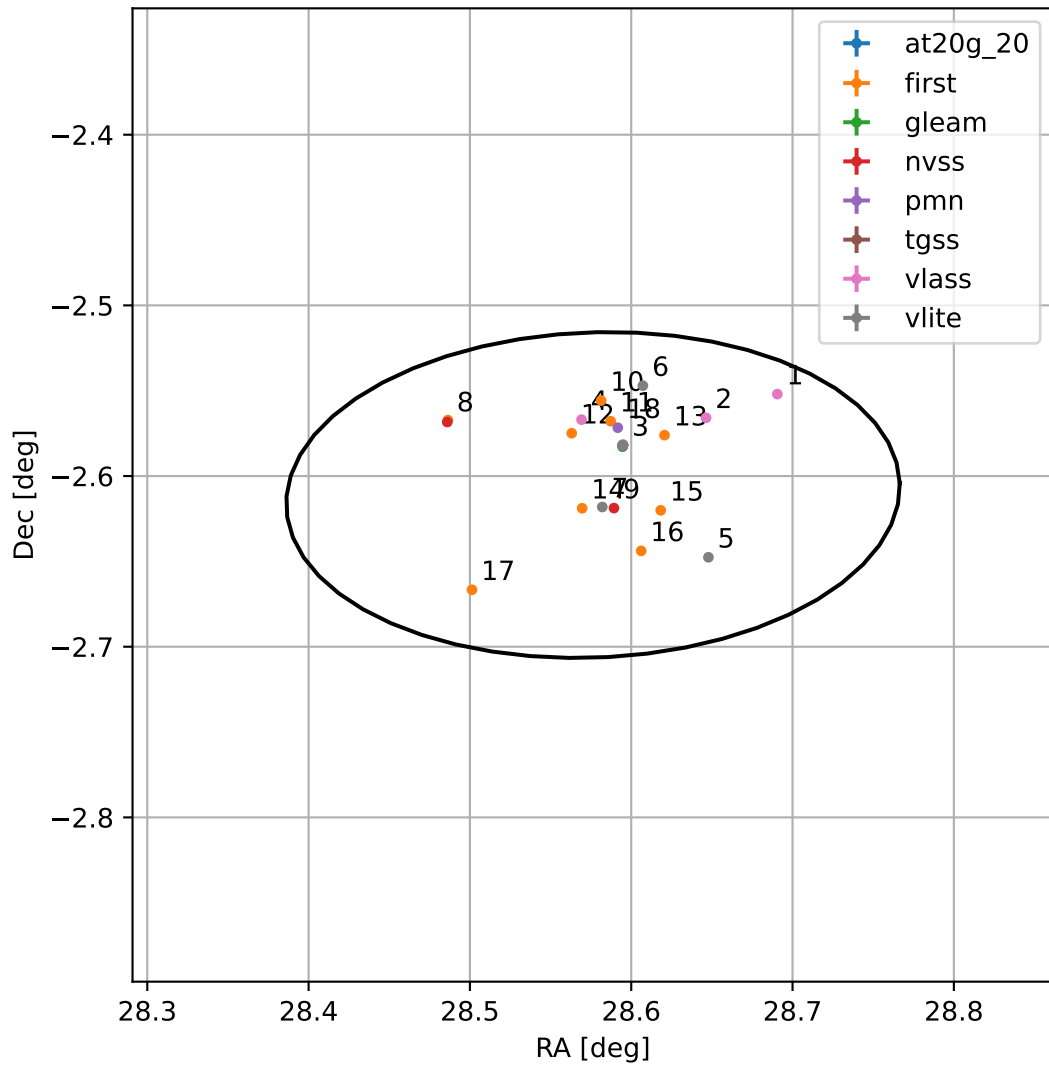
4FGL J0154.3-0236
