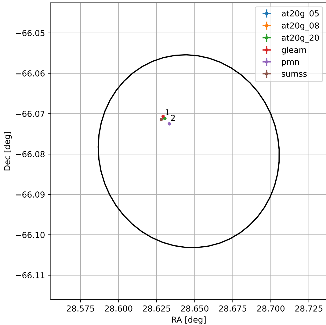
4FGL J0154.5-6604
