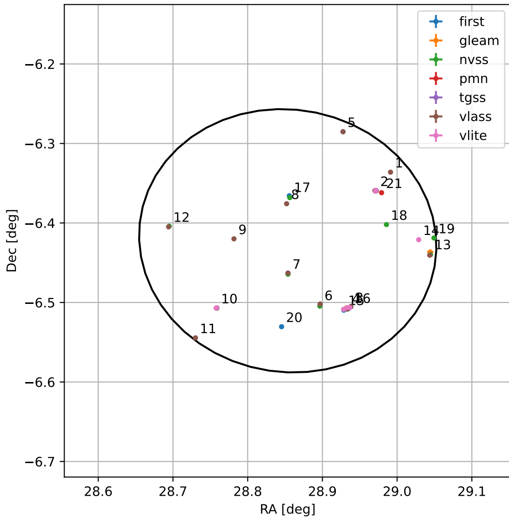
4FGL J0155.4-0625
