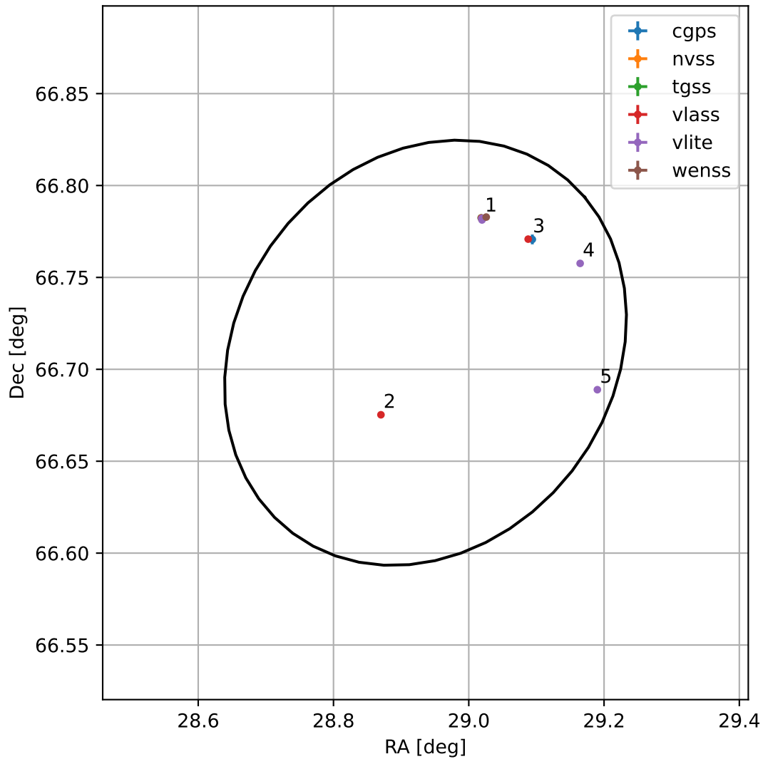
4FGL J0155.7+6642
