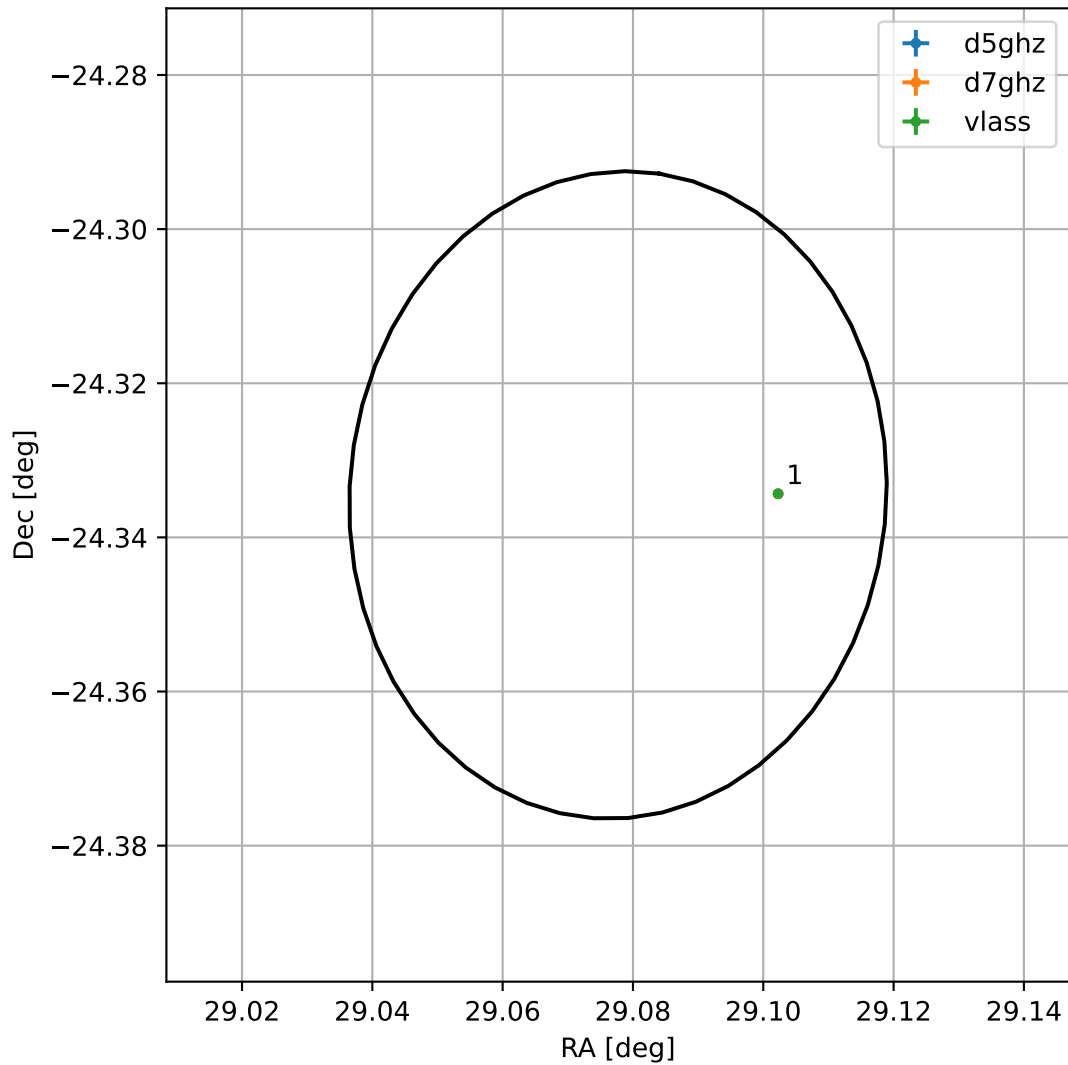
4FGL J0156.3-2420
