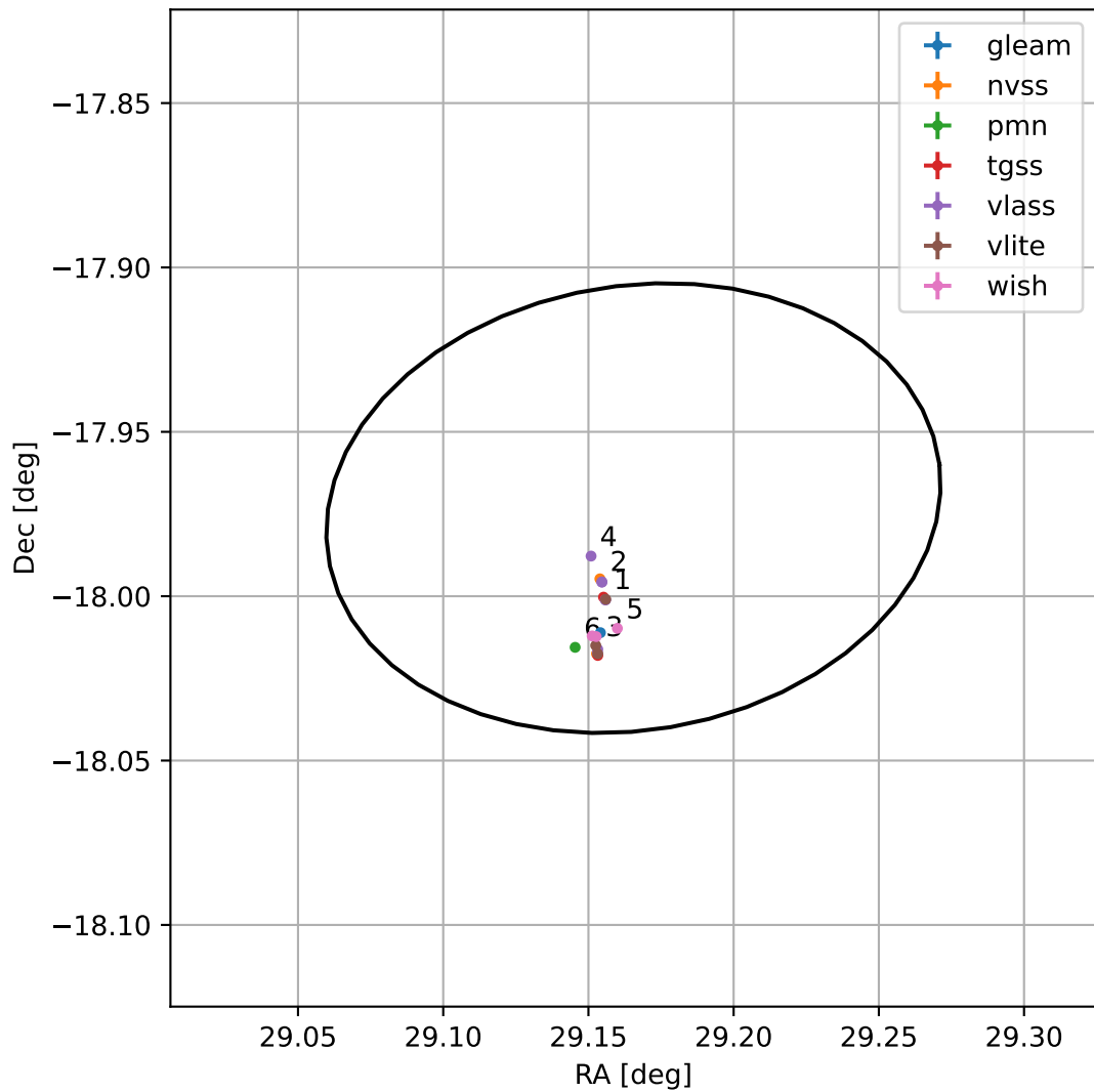
4FGL J0156.6-1758
