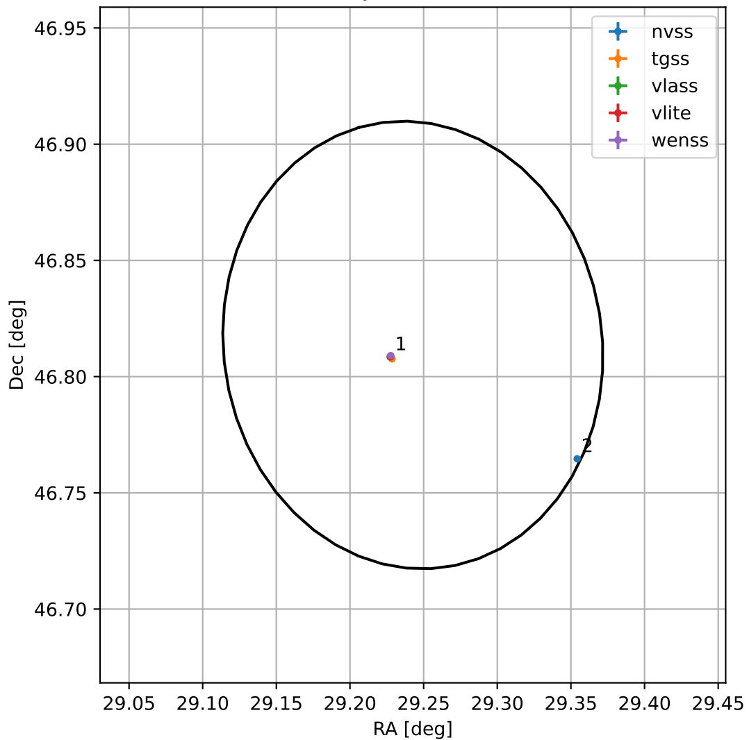
4FGL J0156.9+4648
