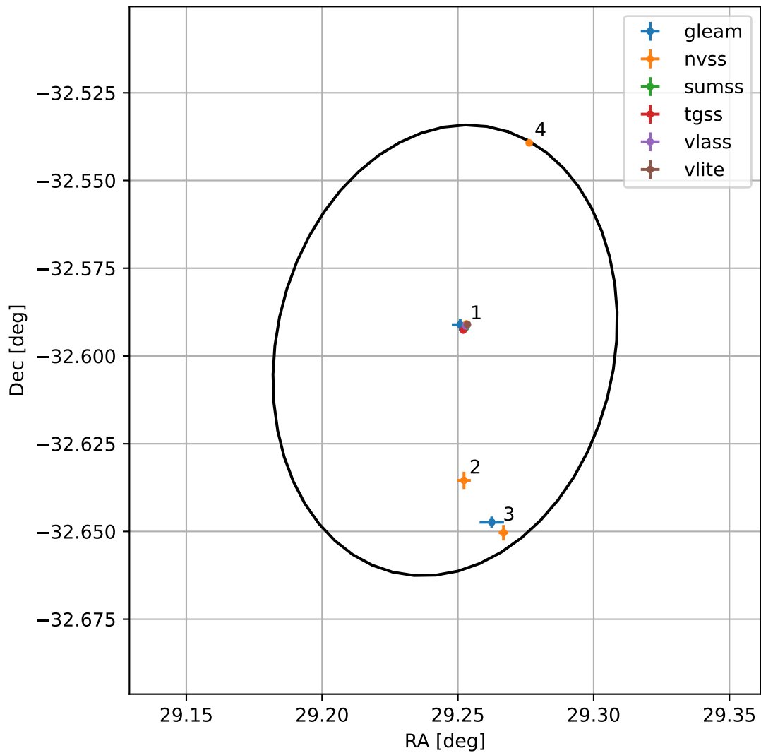
4FGL J0156.9-3235
