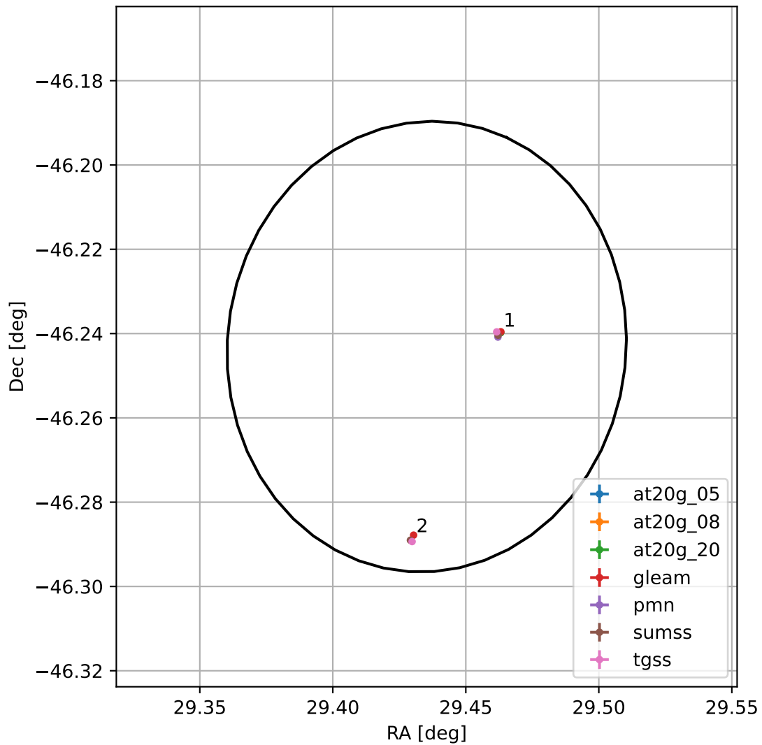
4FGL J0157.7-4614
