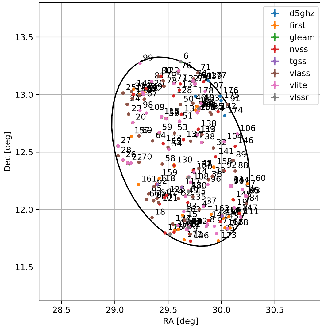
4FGL J0158.4+1230
