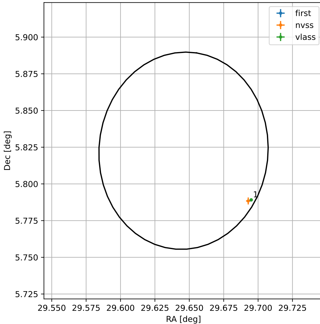
4FGL J0158.5+0549
