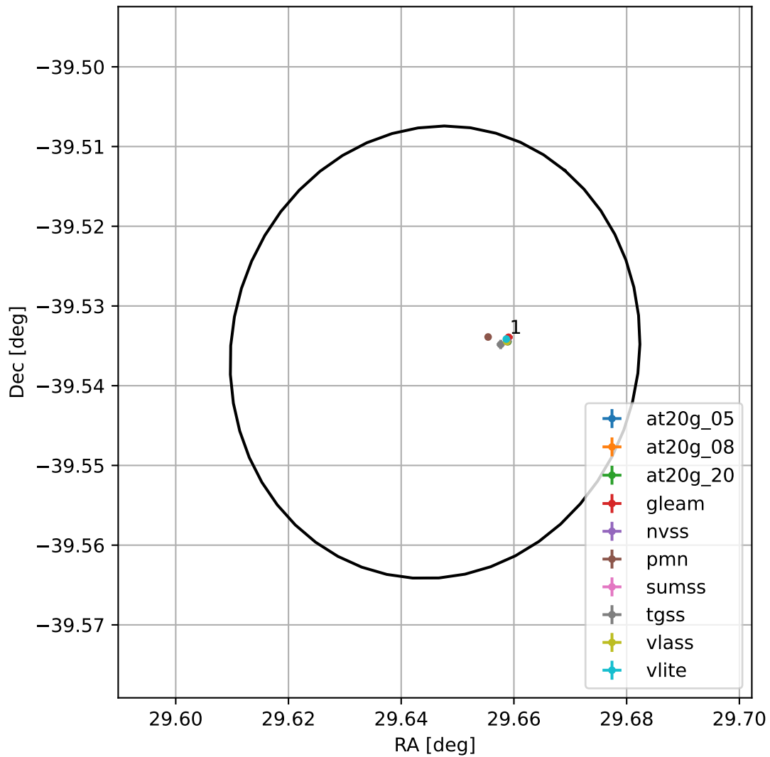
4FGL J0158.5-3932
