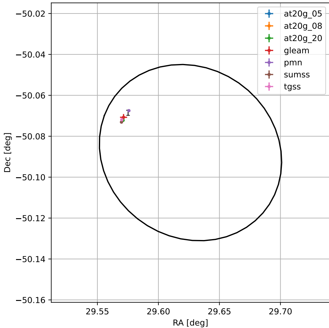
4FGL J0158.5-5005
