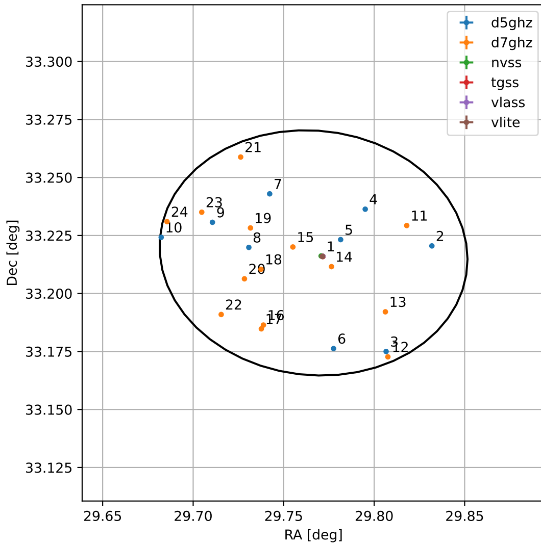
4FGL J0159.0+3313
