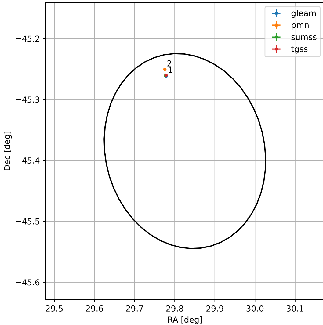
4FGL J0159.3-4523
