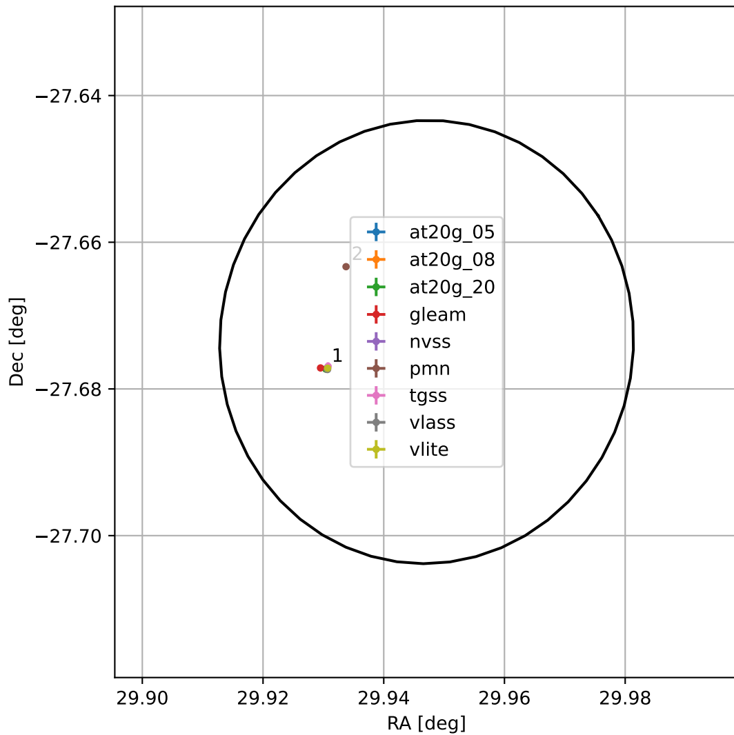
4FGL J0159.7-2740
