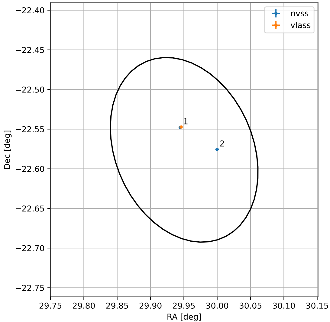
4FGL J0159.8-2234
