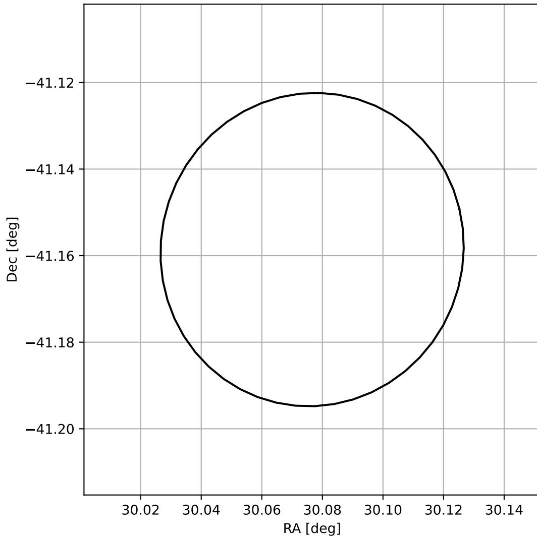
4FGL J0200.3-4109
