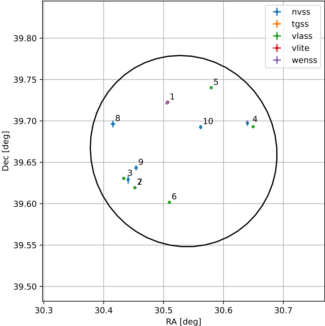
4FGL J0202.1+3939
