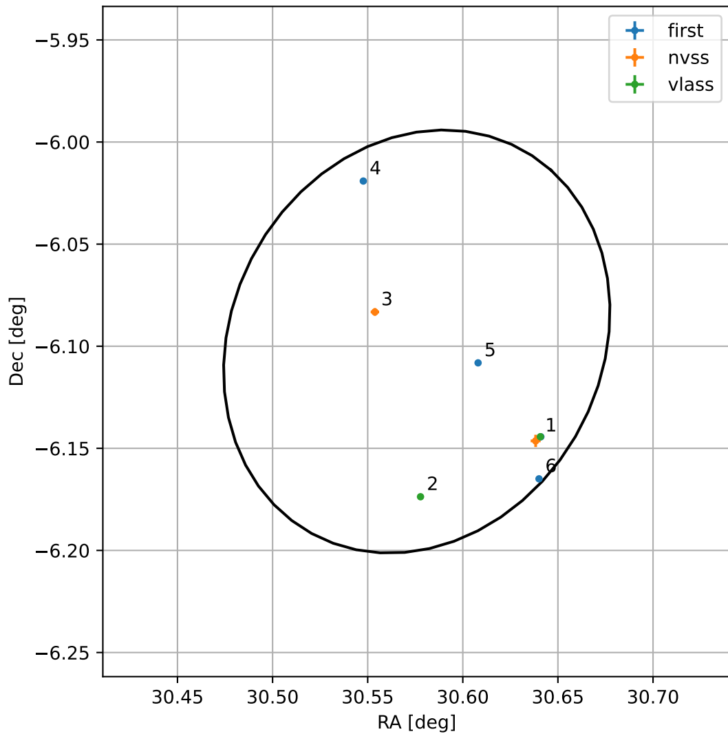
4FGL J0202.3-0605
