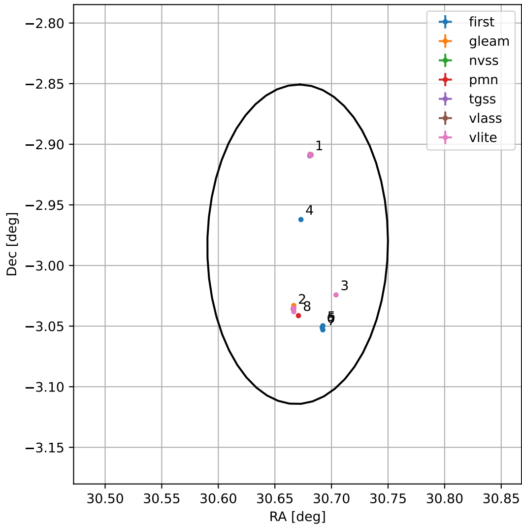
4FGL J0202.6-0258
